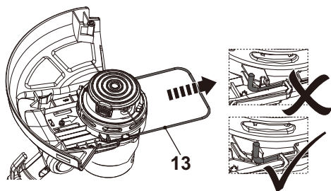
Fig. 10, trimming / edging position
